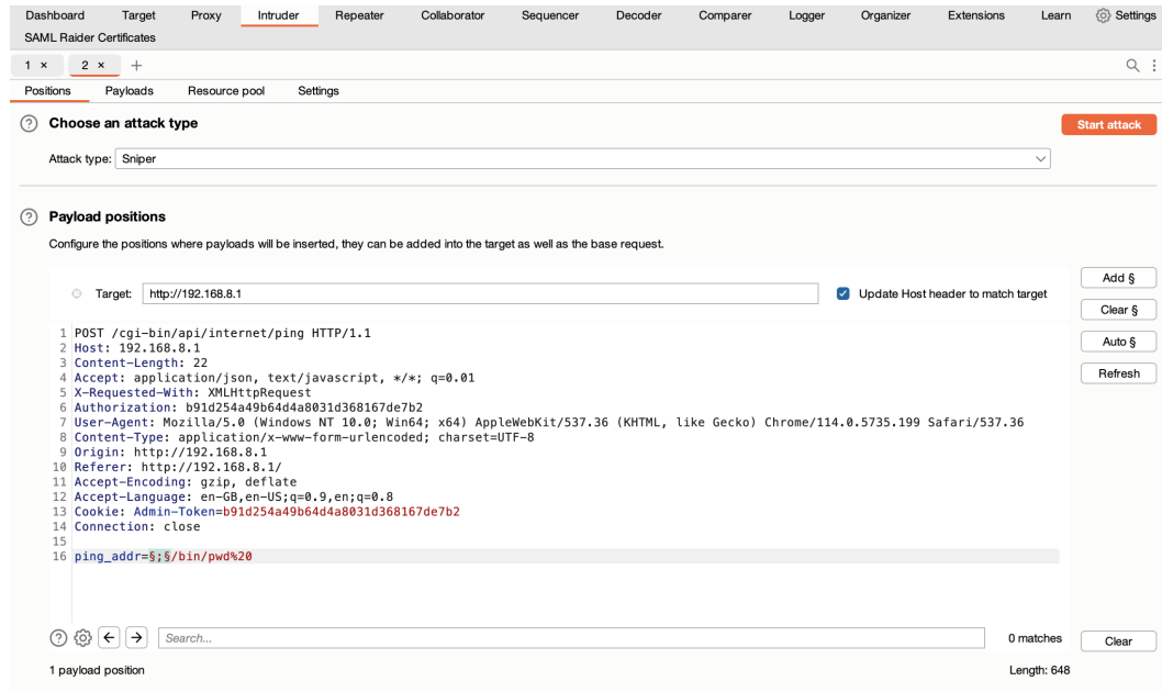
Figure 5.16 – Burp intruder – positions configured
