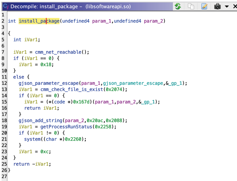
Figure 5.22 – The install_package function
