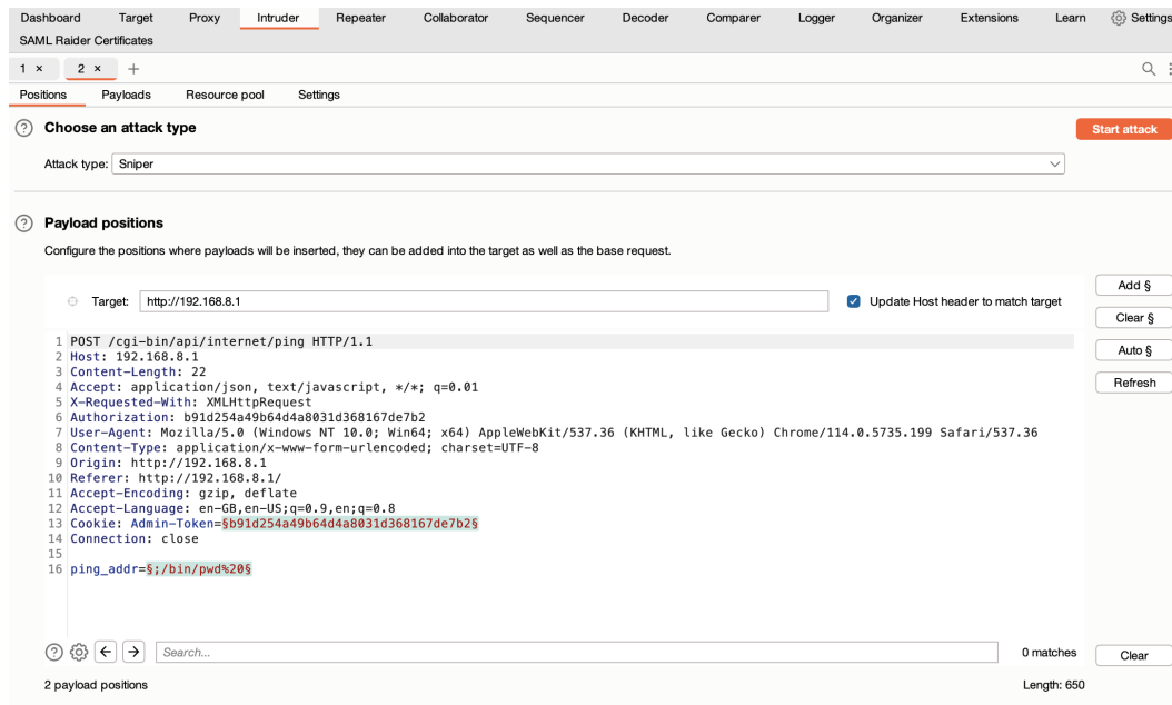
Figure 5.15 – Burp intruder – positions
