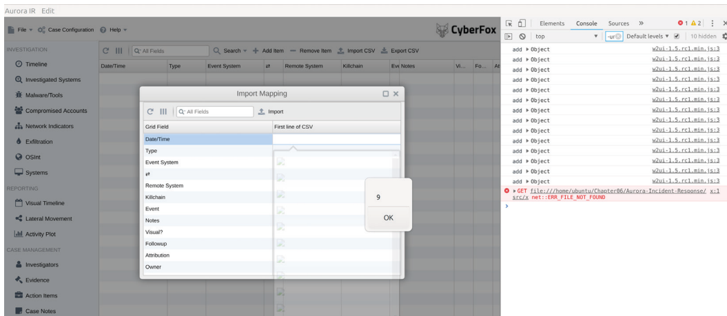
Figure 6.35 – XSS triggered in the Import window
